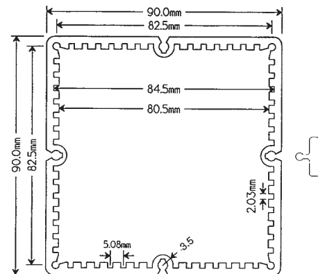
Enclosure Profile
